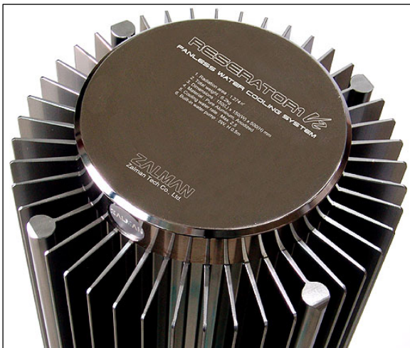
Figure 2: close up of the convective cooling of the reserator.
