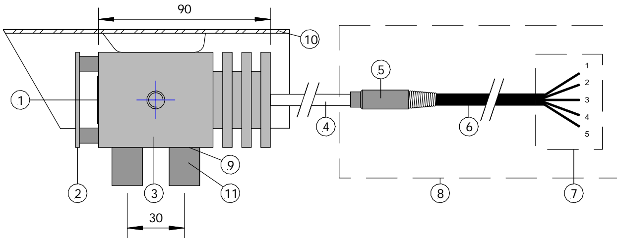
Figure 1 HF02 overview: HF02 consists of a sensor (1) with both temperature and heat flux output, a body (3), a radiation screen (2) and radiation / rain screen (10) to protect the sensor against the environment, a mineral insulated cable (4), potting (5), a plastic cable (6), mounting holes (3/8 UNC) (9) and spacers (11). Area 8 must be between -20 and +70 degrees C, and area 7 must be certified according to the area of installation of the connection box, both within the responsibility of the user. All dimensions are in mm.
